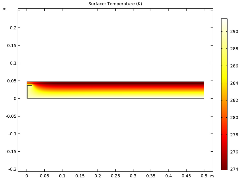
Figure 2: Temperature distribution of ISO 10211:2007 test case 2.
