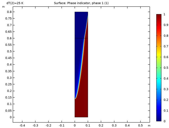
Figure 3: The fraction of liquid phase for \Delta T = 25\text{ K} shows a sharp transition between the liquid and solid phase.
