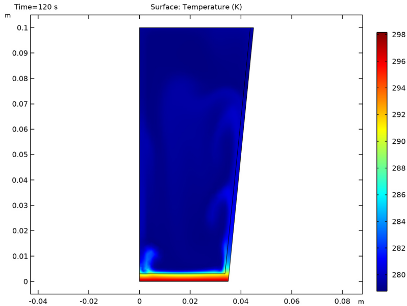
Figure 5: Temperature distribution at time 2 minutes.
