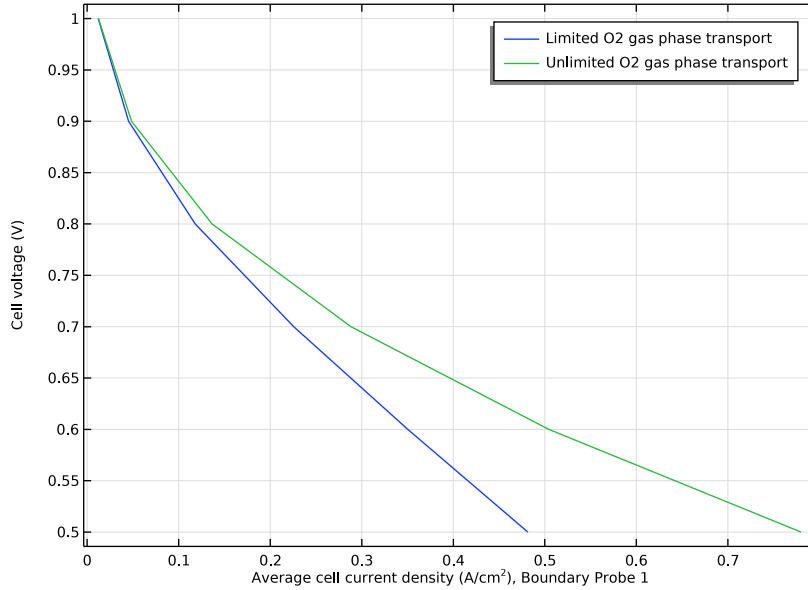
Figure 3: Polarization plot.
