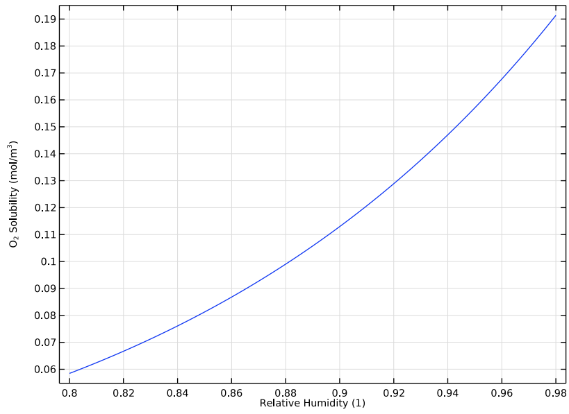
Figure 3: Oxygen solubility vs relative humidity. (Ref. 1)
