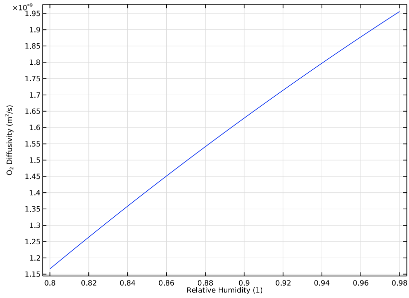
Figure 4: Oxygen diffusivity vs relative humidity. (Ref. 2)
