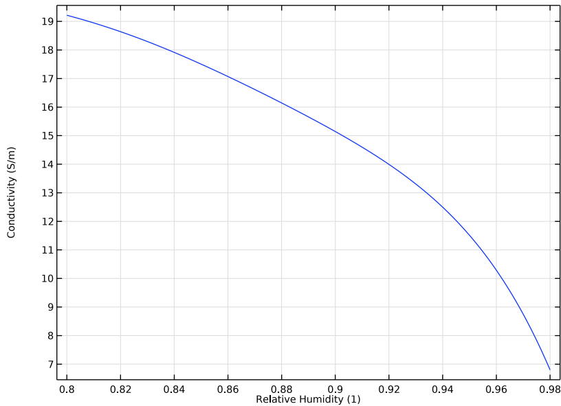
Figure 5: Electrolyte conductivity vs relative humidity. (Ref. 1)
