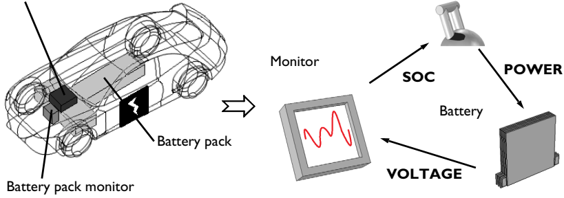
Figure 1: Electric vehicle with key components within the battery management system visualized. As the flowchart shows to the right, the battery voltage is often monitored and from this the SOC is either computed or determined from empirical data. The information from the monitor determines how the control unit will regulate the battery.
