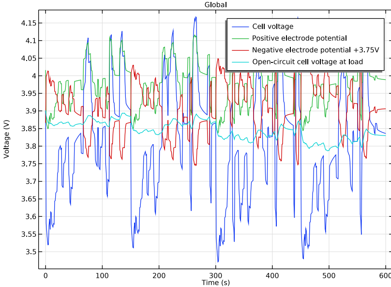
Figure 3: Cell voltage and open-circuit cell voltage, together with electrode potential during drive cycle.
