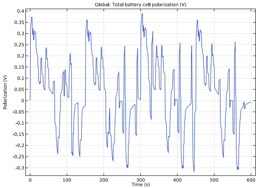
Figure 4: Total polarization during drive cycle.
