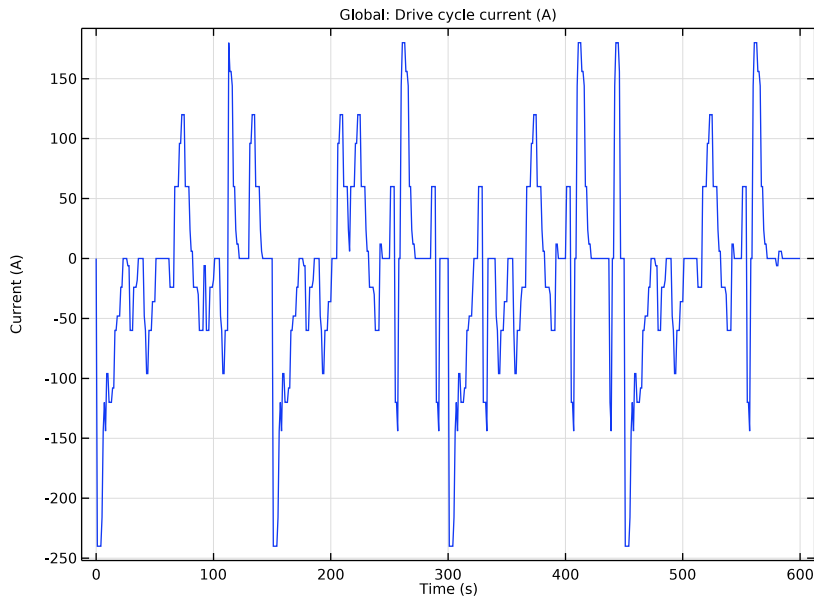
Figure 2: Drive cycle used in the model.
