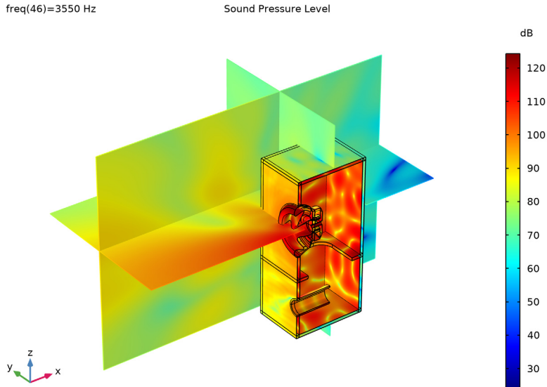
Figure 6: Sound pressure level at 3550 Hz
