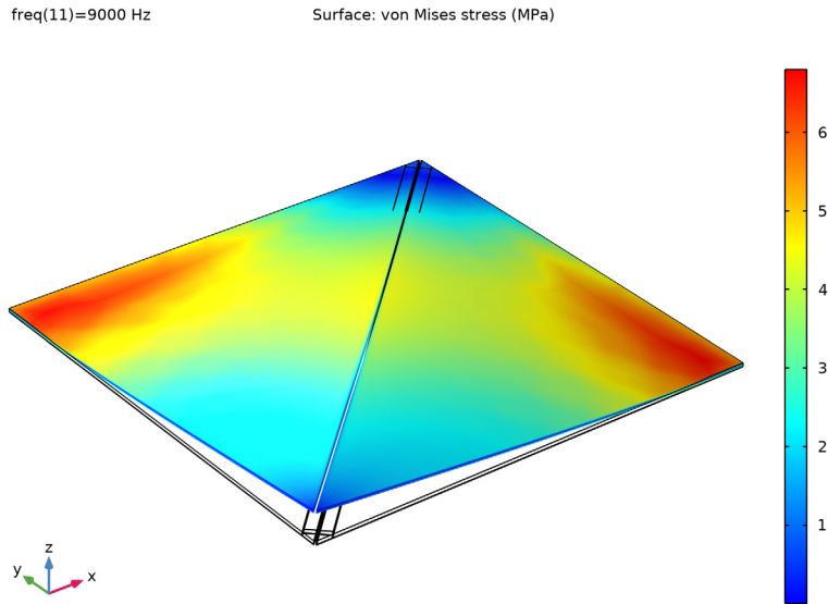
Figure 2: Harmonic part of the von Mises stress at the membranes.
