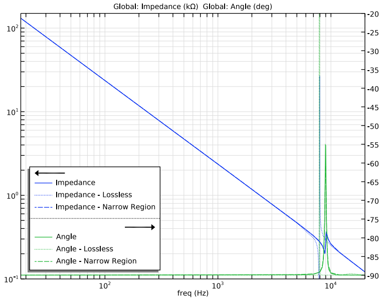
Figure 7: Electric impedance of the speaker, magnitude and phase. The figure also includes the results of a lossless model (pure Pressure Acoustics) and a Pressure Acoustics models with Narrow Region Acoustics.
