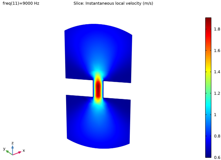
Figure 5: Instantaneous local velocity at 9 kHz.
