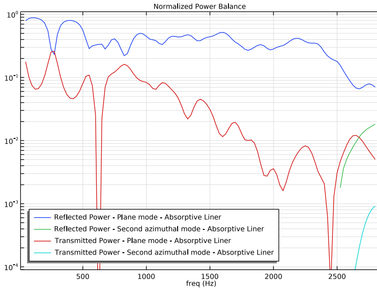
Figure 5: Normalized power balance for the muffler with absorptive lining.
