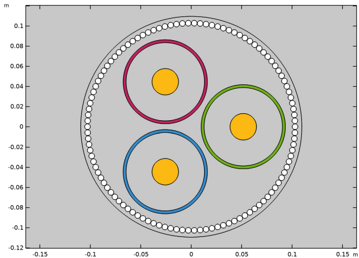
Figure 1: The simplified cable cross section, including the three phases (yellow), the screens (red, green, and blue), and the armor (white).
