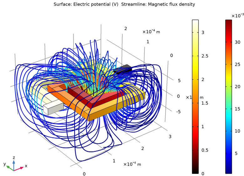
Figure 3: Electric potential in the device and magnetic flux lines around the device.
