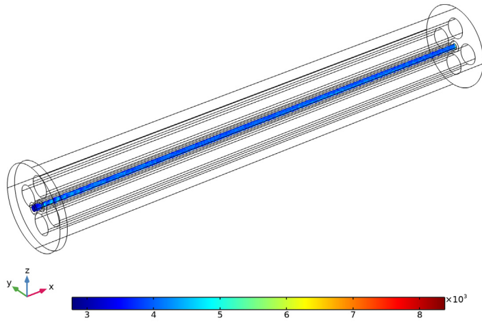
Figure 1: Plot of the particle trajectories inside the quadrupole. The color represents the particle velocity (m/s).
