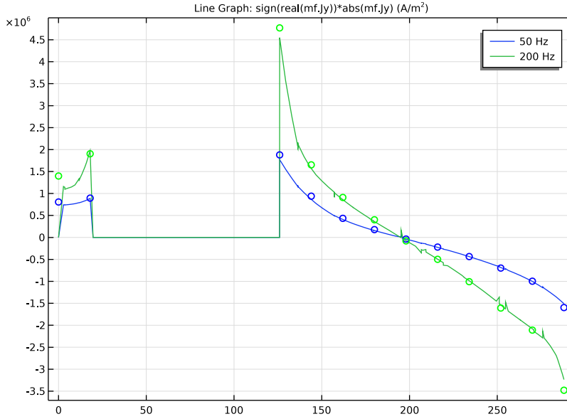
Figure 5: y -components of the induced current densities, J_y ( \text{A/m}^2 ) for 0 \leq x \leq 288 mm at y = 72 mm, z = 19 mm for 50 Hz and 200 Hz. The solid lines are simulation results while the circles are the corresponding measured data from Ref. 1.
