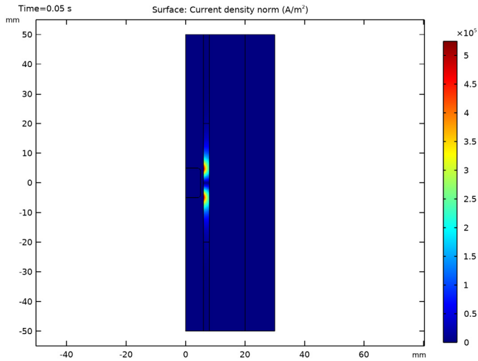
Figure 3: Current density norm at t = 50 ms.
