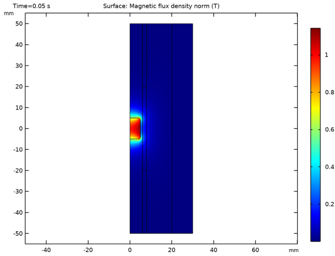
Figure 2: Magnetic flux density norm at t = 50 ms.
