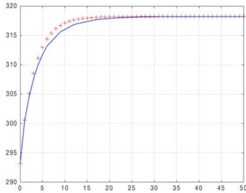
Figure 4-1: Temperature distribution computed with the state-space system (red marker) and COMSOL Multiphysics (blue line).
