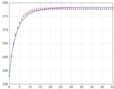
Figure 4-2: Temperature distribution computed with the state-space system 1 (red '+' marker), state-space system without mass matrix (black '.' marker) and COMSOL Multiphysics (blue line).
