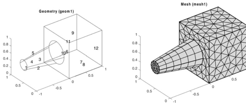
Figure 3-10: Combined structured/unstructured mesh.
