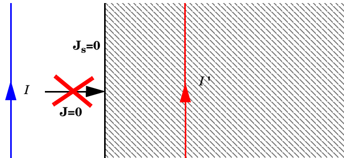
Figure 3-3: The perfect magnetic conductor boundary condition is used on exterior boundaries representing the surface of a high impedance region or a symmetry cut. The shaded (high impedance) region is not part of the model but nevertheless carries effective mirror images of the sources. Note also that any electric current flowing into the boundary is forbidden as it cannot be balanced by induced electric surface currents. The tangential magnetic field vanishes at the boundary. On interior boundaries, the perfect magnetic conductor boundary condition literally sets the tangential magnetic field to zero which in addition to setting the surface current density to zero also makes the tangential electric field (and in dynamics the tangential electric field) discontinuous.
