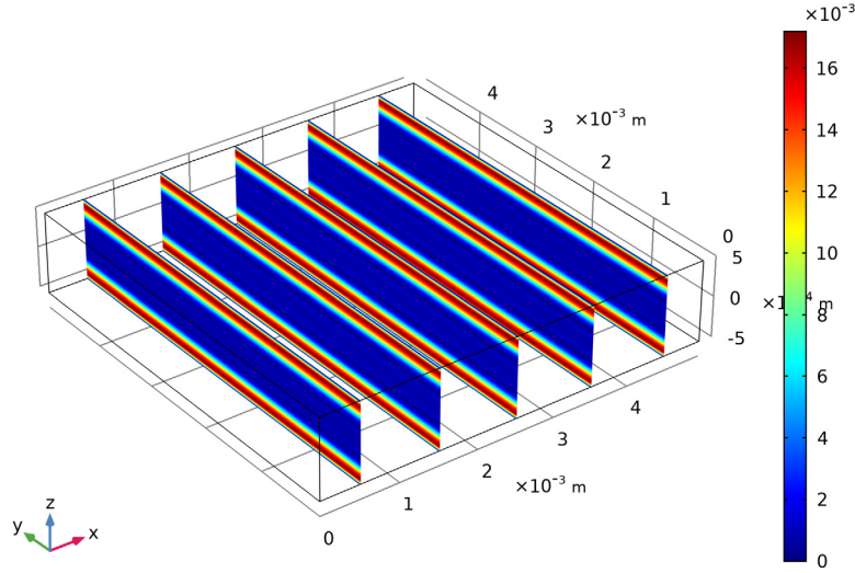
Figure 1: Slice plot of the instantaneous particle velocity U . Outside the boundary layer (red regions) the velocity profile becomes flat as in pressure acoustics.
