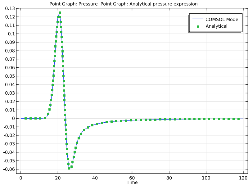
Figure 4: The pressure as function of time at point (x, y) = (20, 10) . The model solution compared to the analytical solution.
