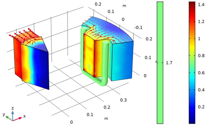
Figure 3: Sector plot of the magnetic flux density. The global coil voltage is represented as a volume plot on the coil itself.
