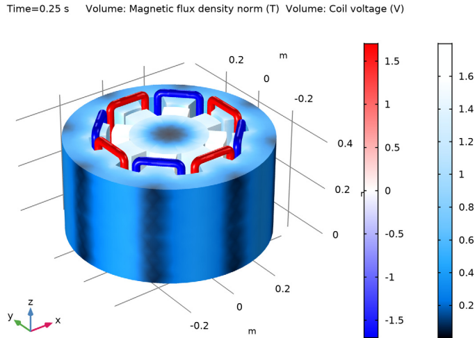
Figure 4: Plot of the magnetic flux density and the global coil voltages in the complete, reconstructed geometry.
