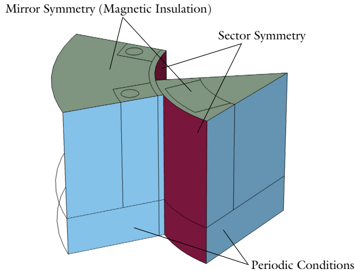
Figure 2: Boundary conditions used to take into account the model symmetry.
