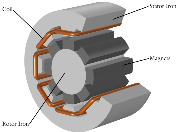
Figure 1: Geometry of the generator.
