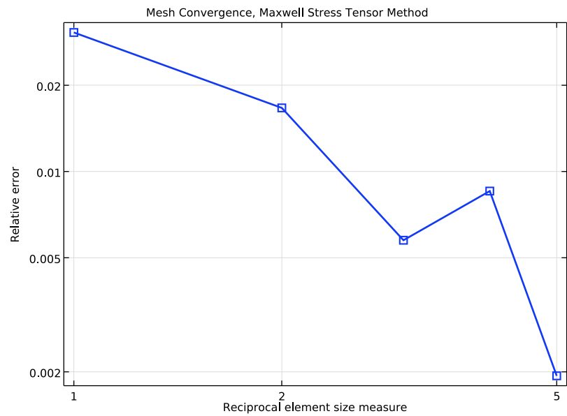
Figure 1: Mesh convergence is shown for the force computation using the Maxwell surface stress method.
