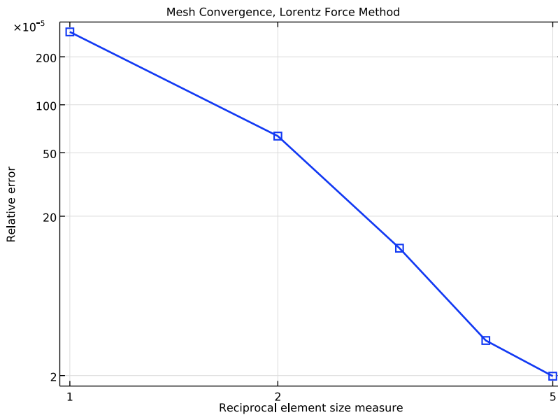
Figure 2: Mesh convergence is shown for the force computation using the volumetric Lorentz force method.
