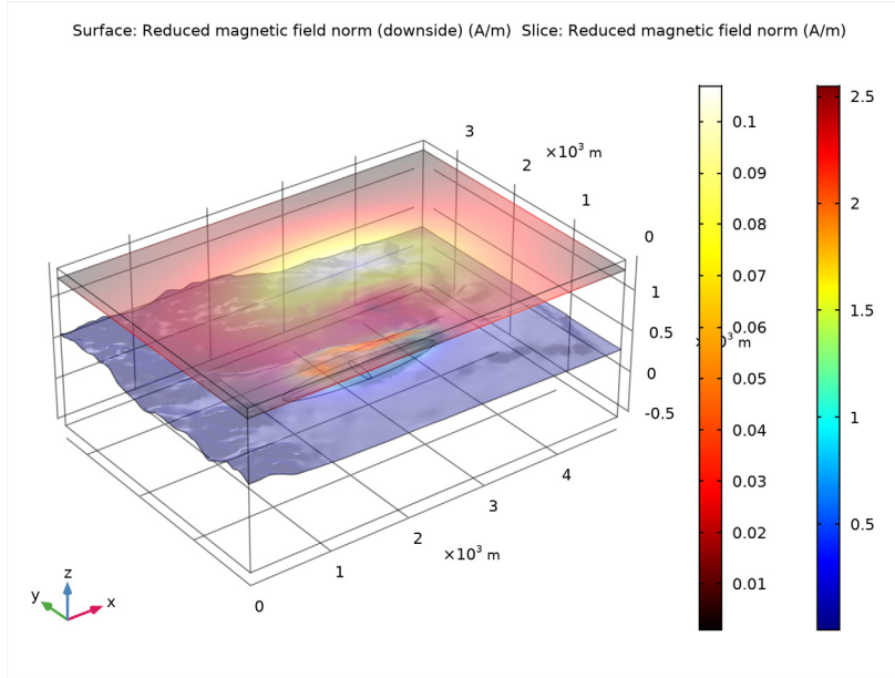
Figure 3: The slice color plot shows perturbations of magnetic intensity (norm of reduced magnetic field) at an altitude 1300 m. The boundary plot shows the same quantity on the ground.
