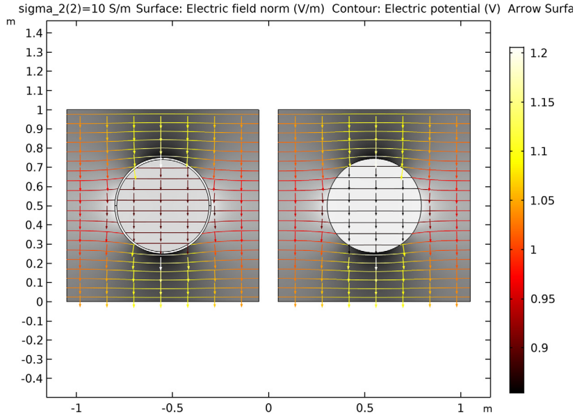
Figure 3: For the case of a thin layer of material that has conductivity ten times greater than the surrounding material.
