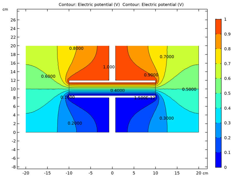
Figure 3: Contours of the voltage field at a slice through the center of the capacitor.
