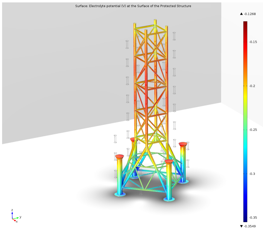
Figure 2: Electrolyte potential at the surface of an oil rig structure.
