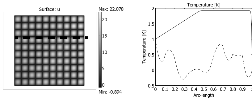
Figure 3-27: Equation 3-5 solved using unstabilized Galerkin formulation. The right plot compares the unstabilized solution (dashed line) along the dashed line in the left plot ( y = 0.8 ) with the reference solution (solid line).
