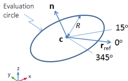
Figure 21-5: Schematic of the evaluation circle used in the Directivity and Radiation Pattern plots, showing the circle center \mathbf{c} , evaluation plane normal \mathbf{n} , evaluation radius R , and reference direction \mathbf{r}_{\text{ref}} .
