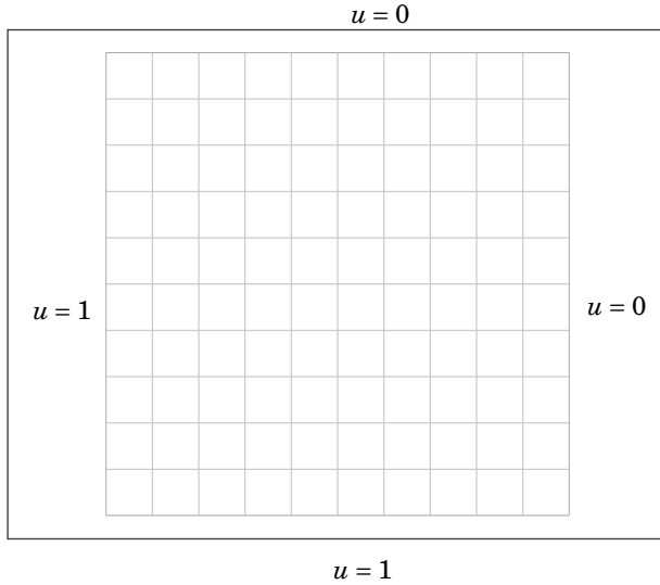
Figure 3-25: The computation domain, mesh, and boundary condition for Equation 3-5.
