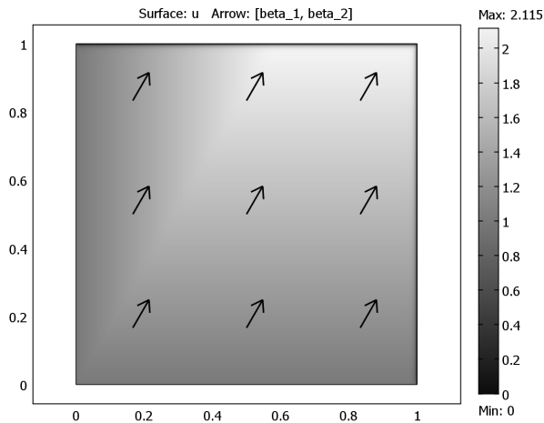
Figure 3-26: Reference solution of Equation 3-5. Solved using 100 times 100 quadratic elements with streamline diffusion and crosswind diffusion.
