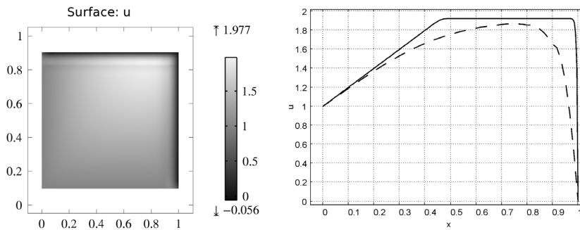
Figure 3-28: Equation 3-5 solved using isotropic diffusion. The right plot compares the stabilized solution (dashed line) along y = 0.8 with the reference solution (solid line).
