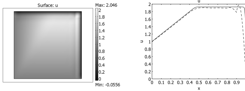
Figure 3-29: Equation 3-5 solved using streamline diffusion. The right plot compares the stabilized solution (dashed line) along y = 0.8 with the reference solution (solid line).
