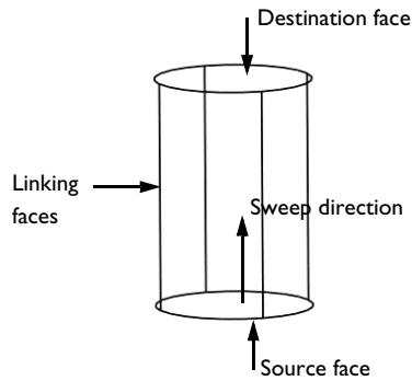
Figure 8-2: Classification of the boundaries about a domain used for swept meshing.
