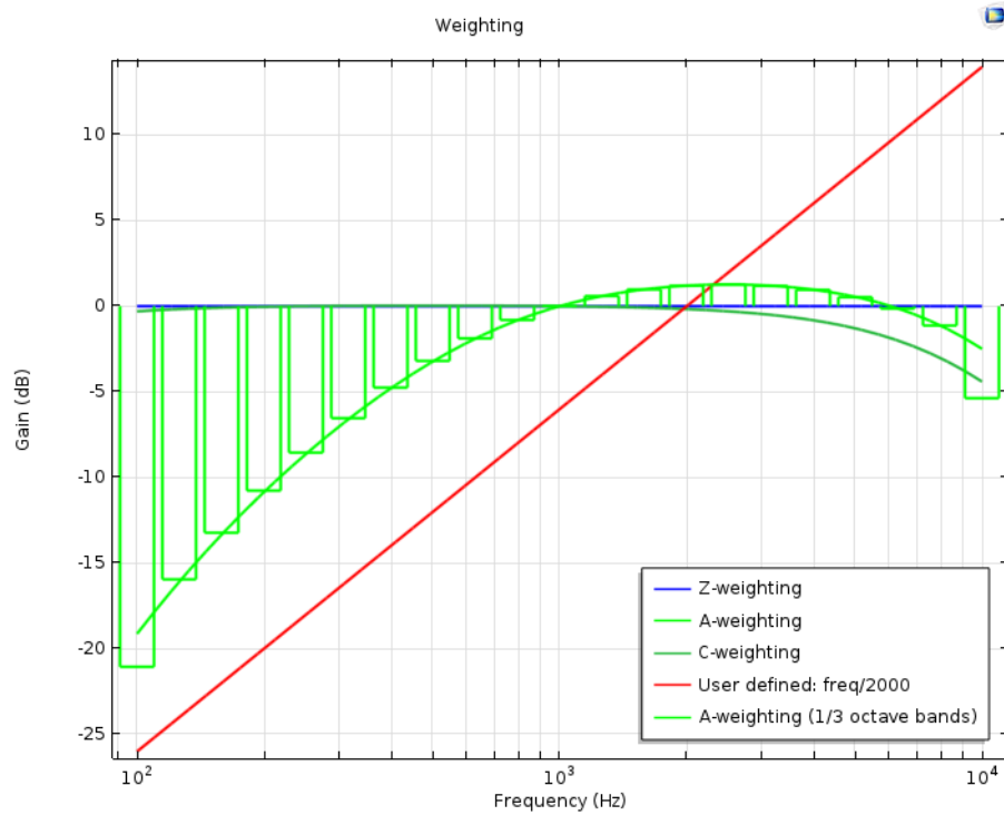
Figure 21-7: The plot shows Z-weighting (blue), A-weighting (light green), C-weighting (dark green), and a user-defined weighting (red). The 1/3 octave bands (light green) also show A-weighting.
