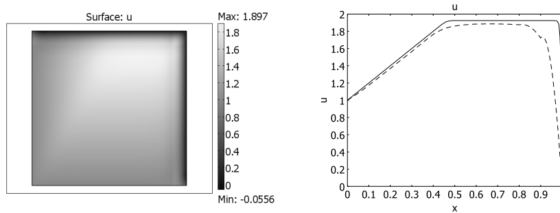
Figure 3-30: Equation 3-5 solved using streamline diffusion and crosswind diffusion. The right plot compares the stabilized solution (dashed line) along y = 0.8 with the reference solution (solid line).
