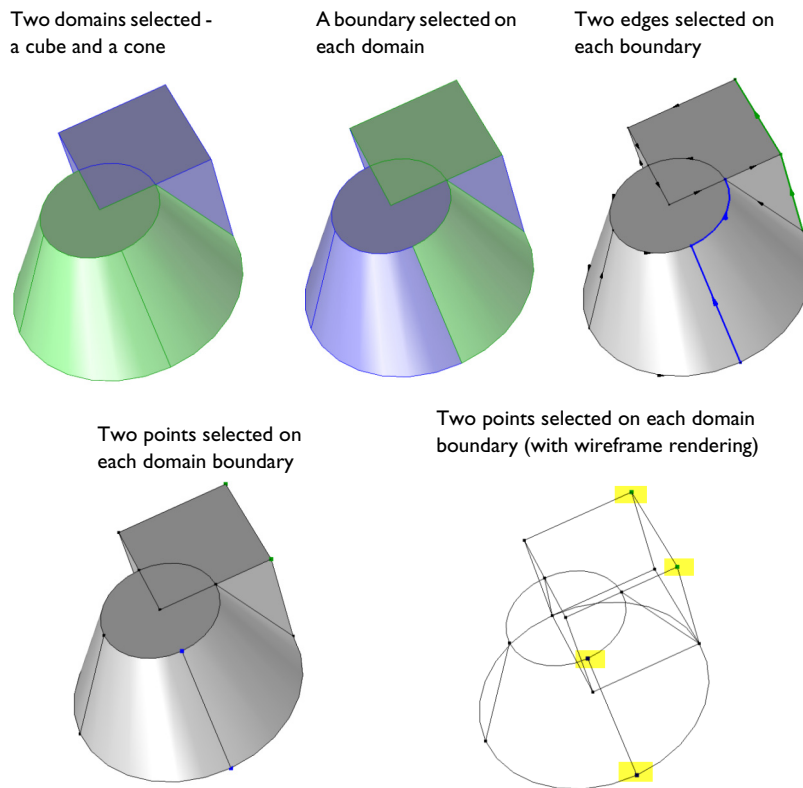
Figure 6-1: A 3D geometry comprises domains, boundaries, edges, and points.
