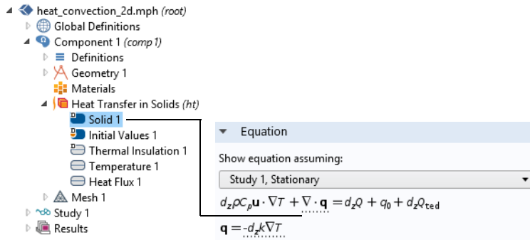
Figure 3-18: The Solid contribution to the equation for a 2D model.
